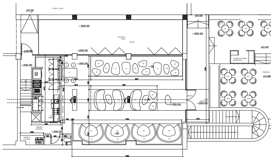
2 Floor Plan SCALE 1:50
